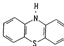
Phenothiazine
